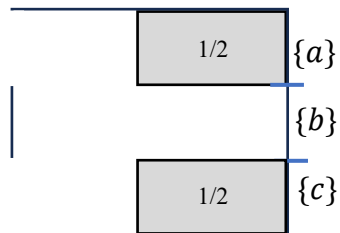
Figure 10: Case 2 hit probabilities with no detection at slits showing characteristic stripes due to destructive interference at \{b\}
