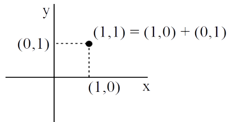
Figure 2: Superposition of definite- or eigen-states is indefinite between them superposition (1,1).
