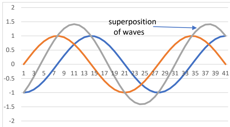
Figure 1: Superposition as addition of definite waves to give definite waves
