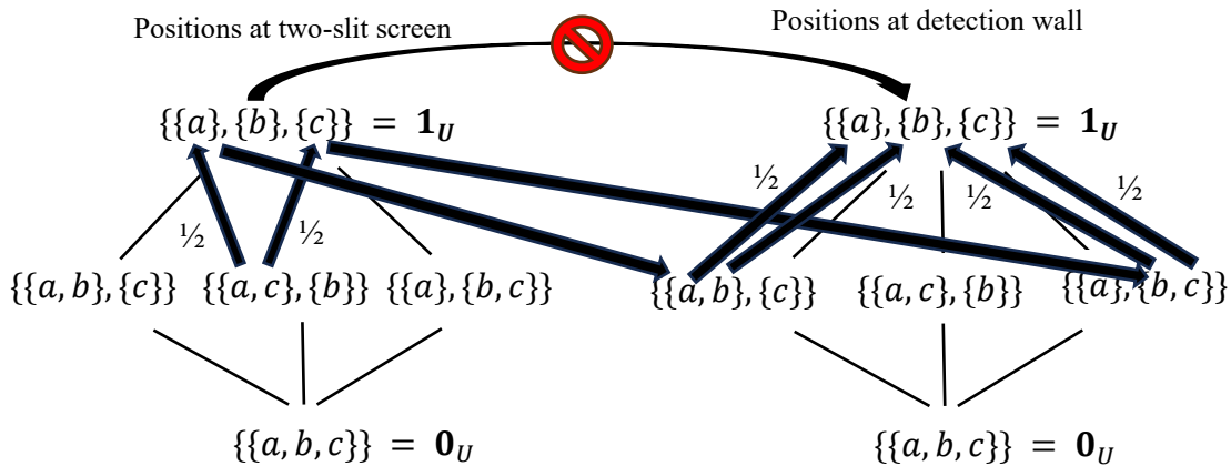
Figure 11: Case 1 evolutions with no spatial (i.e., classical) trajectory from a classical state at the screen to a classical state at the wall
