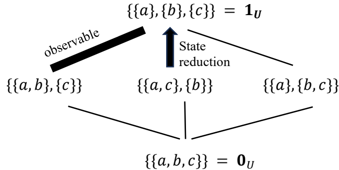
Figure 6: Join of \{\{a, b\}, \{c\}\} and \{\{a, c\}, \{b\}\} to yield \{\{a\}, \{b\}, \{c\}\} = 1_U
