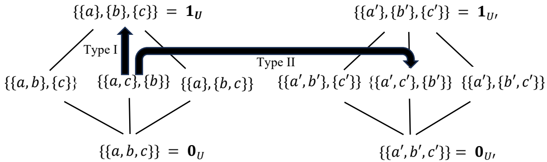
Figure 7: Type I and Type II processes
