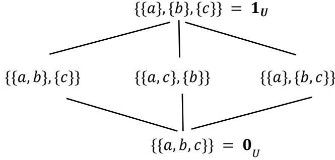
Figure 3: The lattice of partitions on U = \{a, b, c\}
