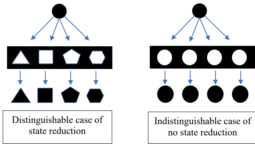
Figure 5: State reduction or not depending on whether the interaction makes distinctions
